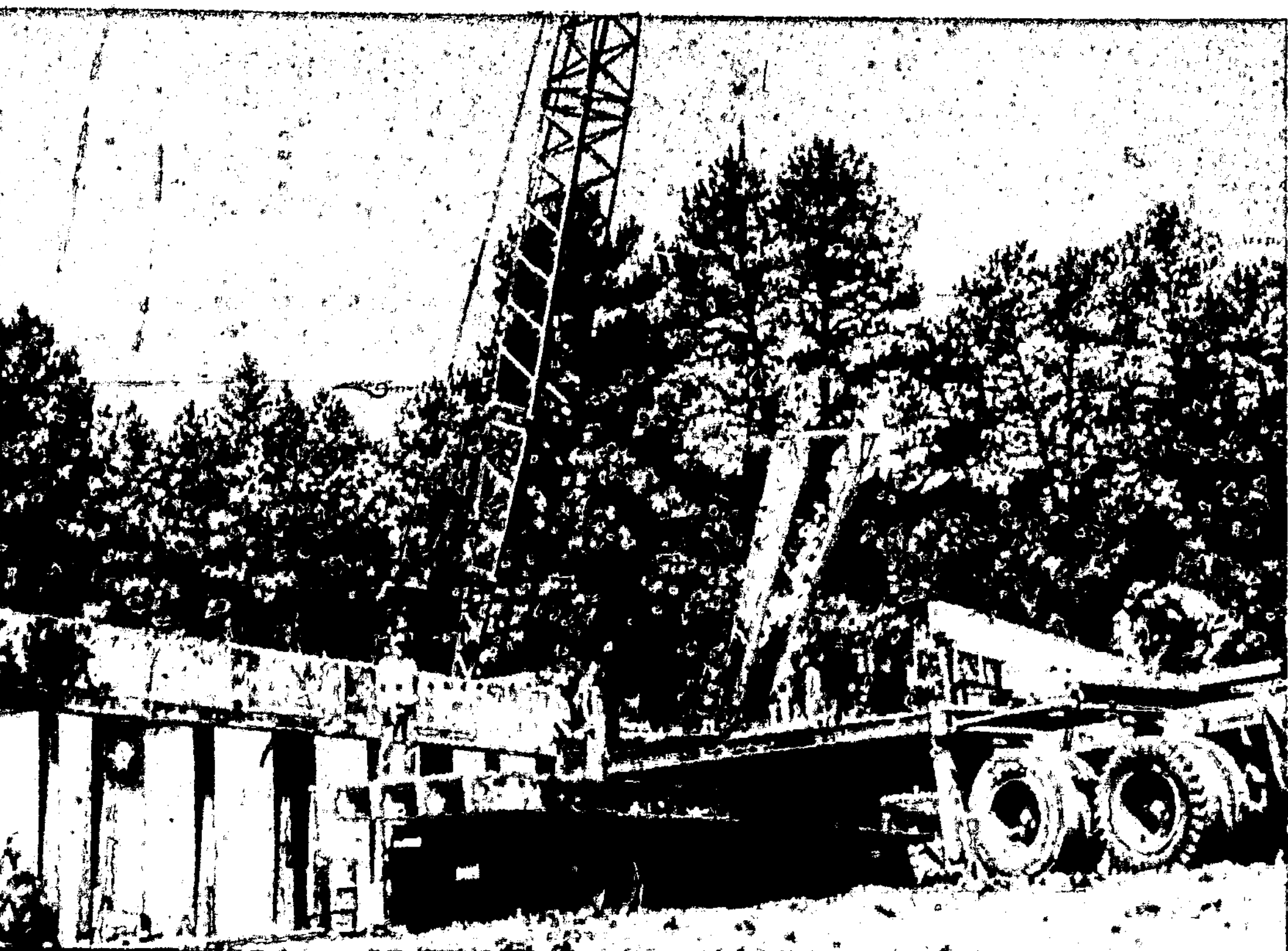
ROOF GOES ON —Prestressed concrete double-T roofing beams 71½ feet long, were installed by a huge crane last week on the new shopping center being built on Sudderth
