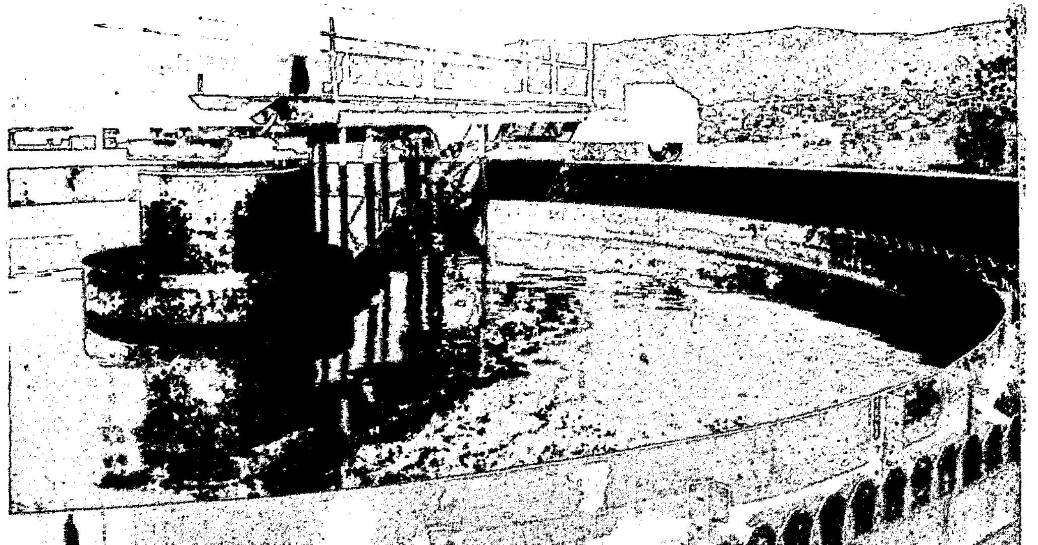
SECONDARY CLARIFIER. After sewage passes through the aeration tanks, it comes to the clarifier for the final step in the treatment process. Here, solid matter settles and clean water spills over the notched barrier and is on its way to chlorination before being discharged into the river.
