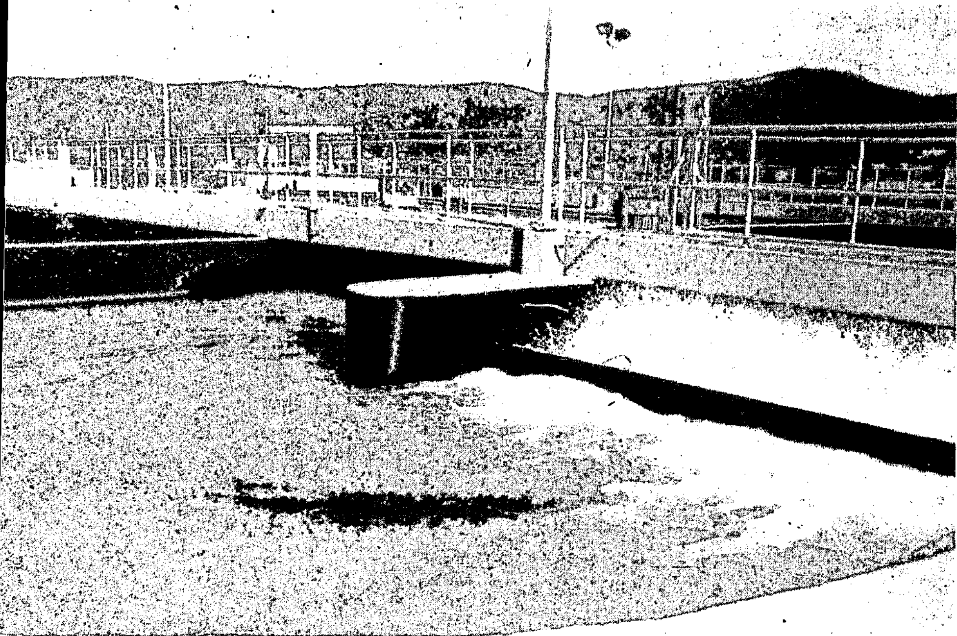
WASTE IS CHURNED in one of four aeration tanks at the new Regional Wastewater Treatment Plant at Biscuit Hill. The plant, which opened last week, is an activated sludge plant. In the aeration tanks, oxygen is supplied to the water to keep bacteria thriving, thereby speeding up the treatment process. Up to 2.6 million gallons can be treated each day at the plant.
